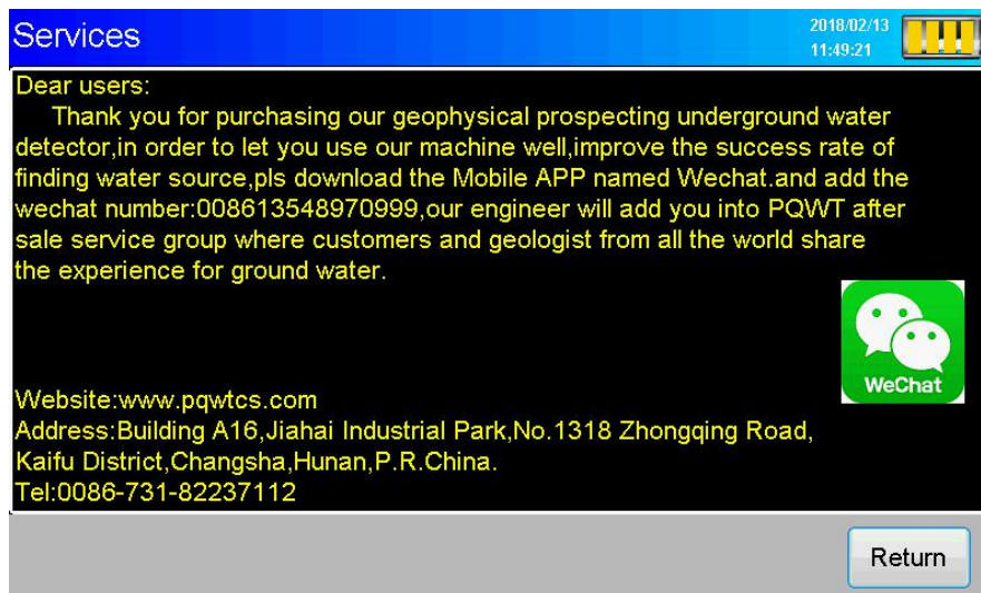
Figure 14 About Screen
