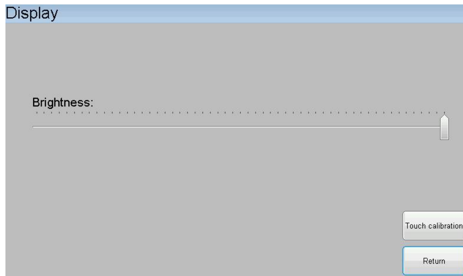
Figure 12 Display screen
